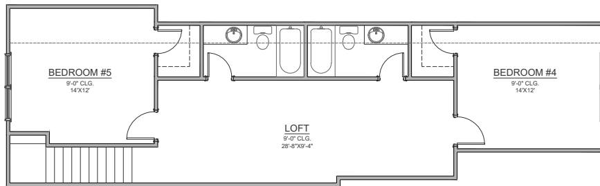
UPPER FLOOR PLAN
