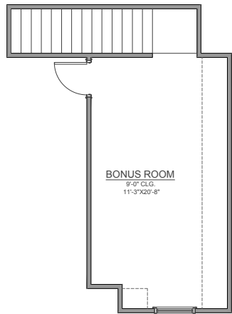
BONUS ROOM PLAN
