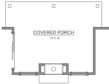
EXTENDED 4' PORCH OPTION
